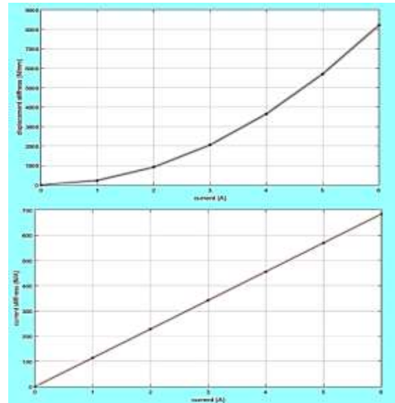
Fig.10. The displacement stiffness and current stiffness vs current
