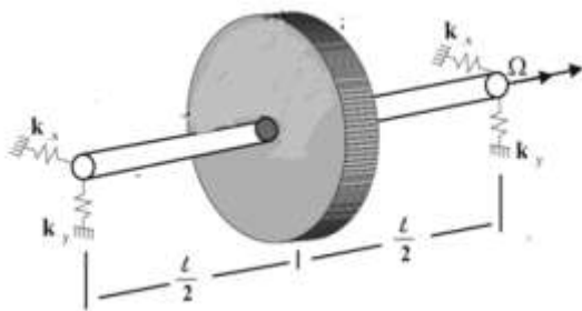
Fig.1. Flexible shaft with rigid disk and flexible bearing
