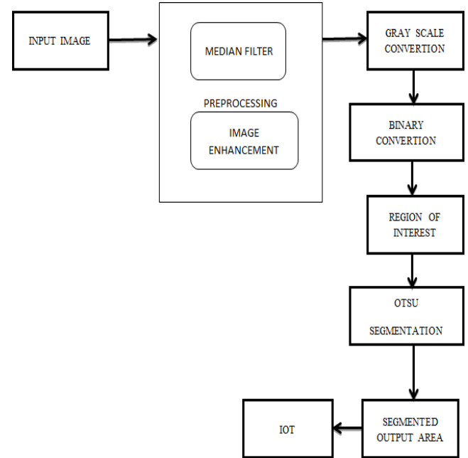
Fig. 2. The Inner Architecture diagram of the proposed pothole detection algorithm
