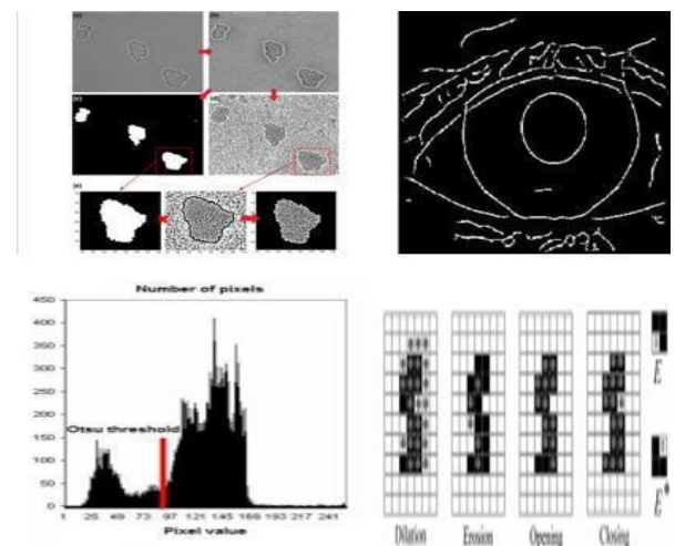
Fig. 4. Techniques of Crack Detection (a) Image Pre-processing, (b) Edge Detection, (c) Image Segmentation, and (d) Morphology.
