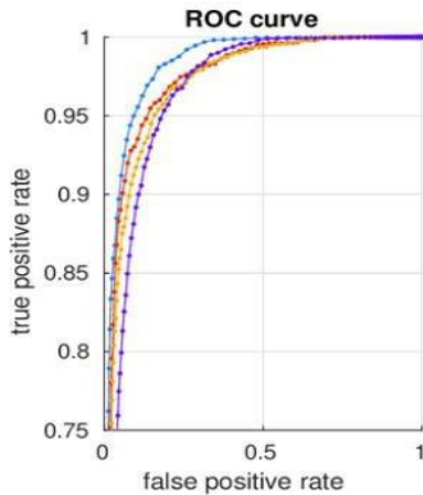
Fig.17. ROC Curve.
