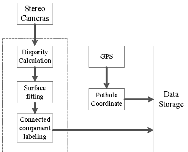
Fig. 1. The block diagram of the proposed pothole detection algorithm.
