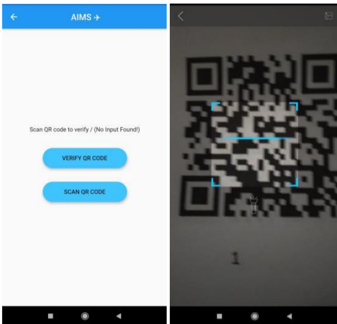
Fig. 6. Home Page
