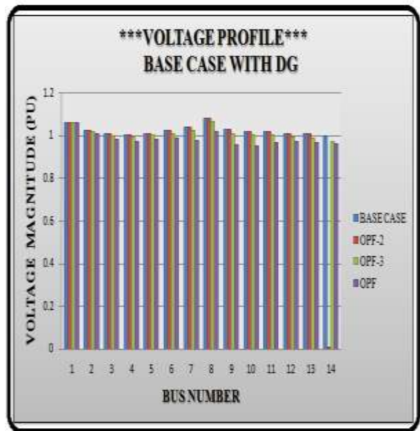
Fig 4: A voltage profile with DG units in the base case.
