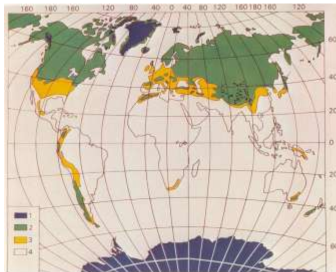
Fig. 1: Map of permanent (blue), relatively stable (green), and seasonal (yellow) global snow cover (Martinec, 1985).
