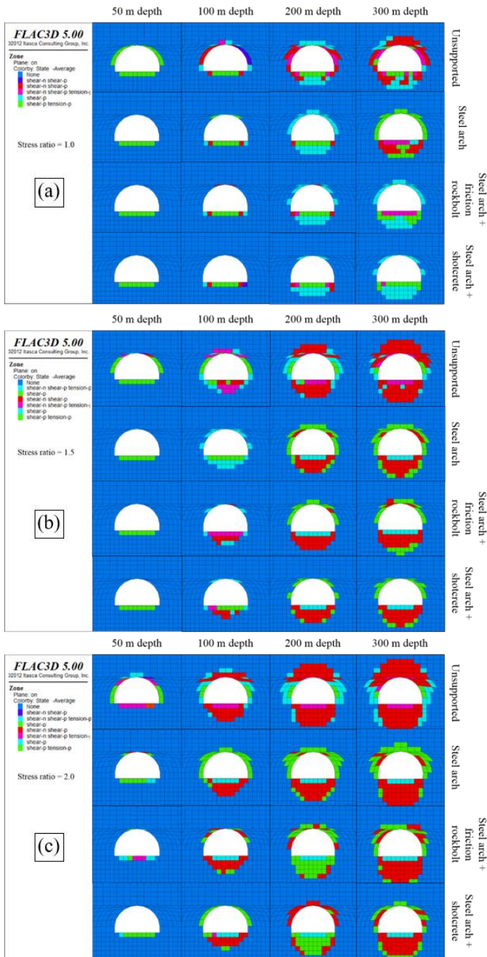
Fig. 14. Failure zone of tunnel after installation of steel arch, and steel arch in combination with friction rockbolt and shotcrete as auxiliary support (a) k = 1.0 (b) k = 1.5 (c) k = 2.0
