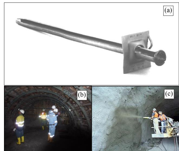
Fig. 11. Support systems for roof and sidewalls of mine tunnel (a) Friction rockbolt (b) Steel arch (c) shotcrete
