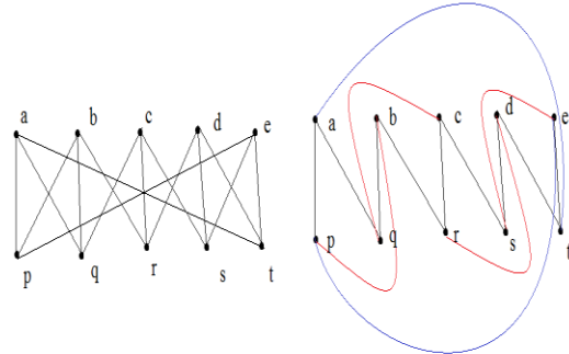
fig:1.1 cubic,3-connected, bipartite graph fig 1.2 cubic, 3-connected, bipartite and non-planar graph
