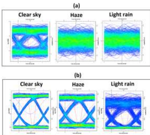
Fig. 8. Eye-opening comparisons (a) without EDFA (b) with
