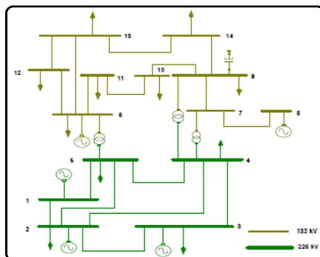
Fig.1:Sample Test system for 14-Bus IEEE
