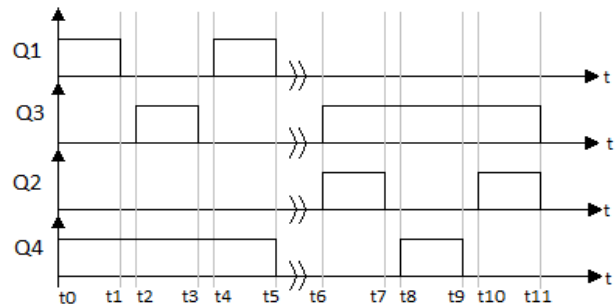
Fig. 3. Control strategy under half cycle modulation.
