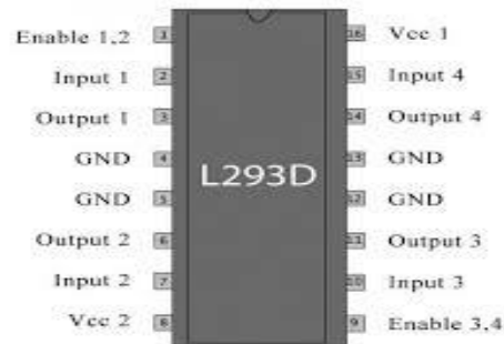
Figure.3 Motor Driver L293D
