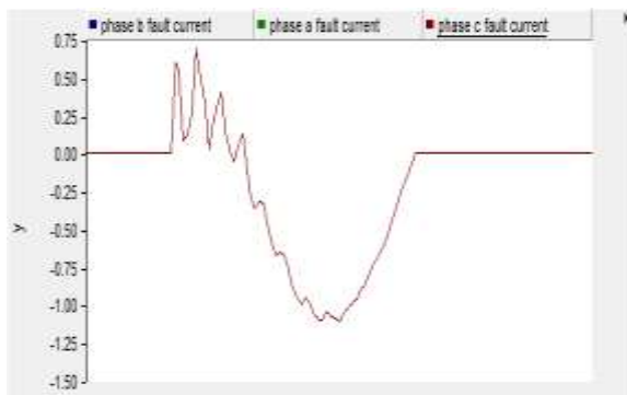
Characteristics of fault current of phase-C
