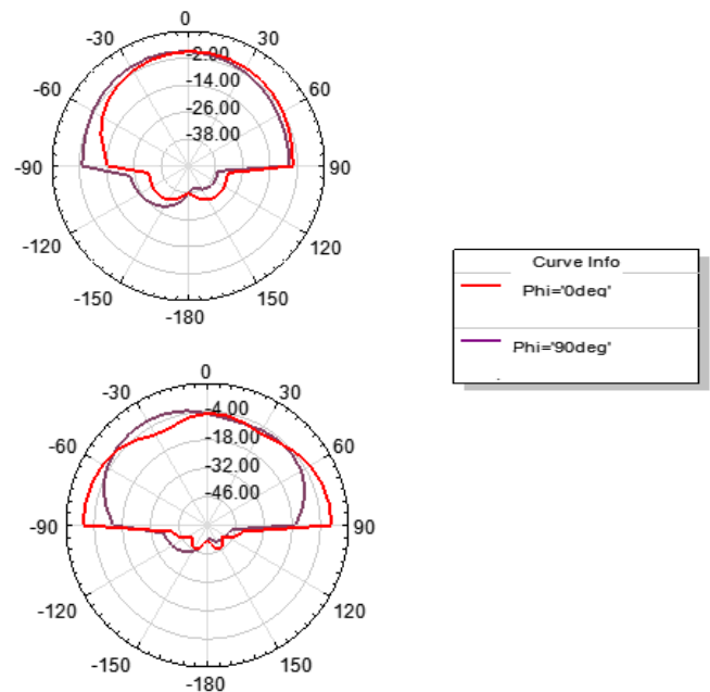
Figure 4. Simulated radiation pattern of 0th iteration at (a) 3.34GHz (b) 7.81GHz
