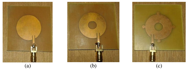
Fig. 7. Fabricated geometry of (a) 0th iteration (b) 1st iteration (c) 2nd iteration
