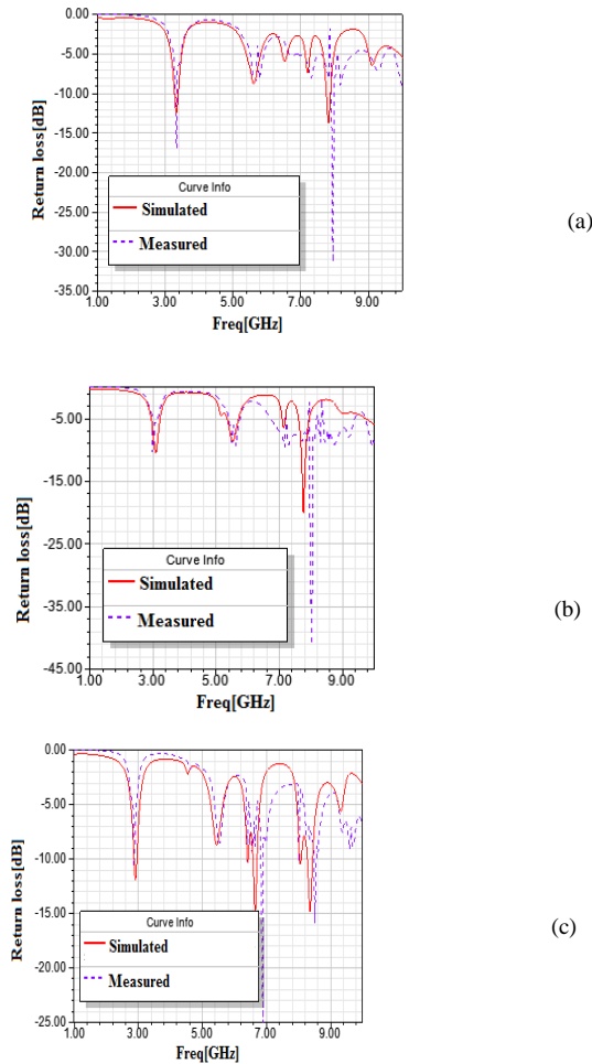
Fig. 9. Simulated and measured return loss vs. frequency plot of (a) 0 th iteration (b) 1 st iteration (c) 2 nd iteration
