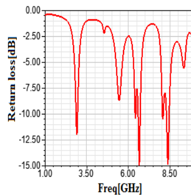
(c) IInd iteration stage
