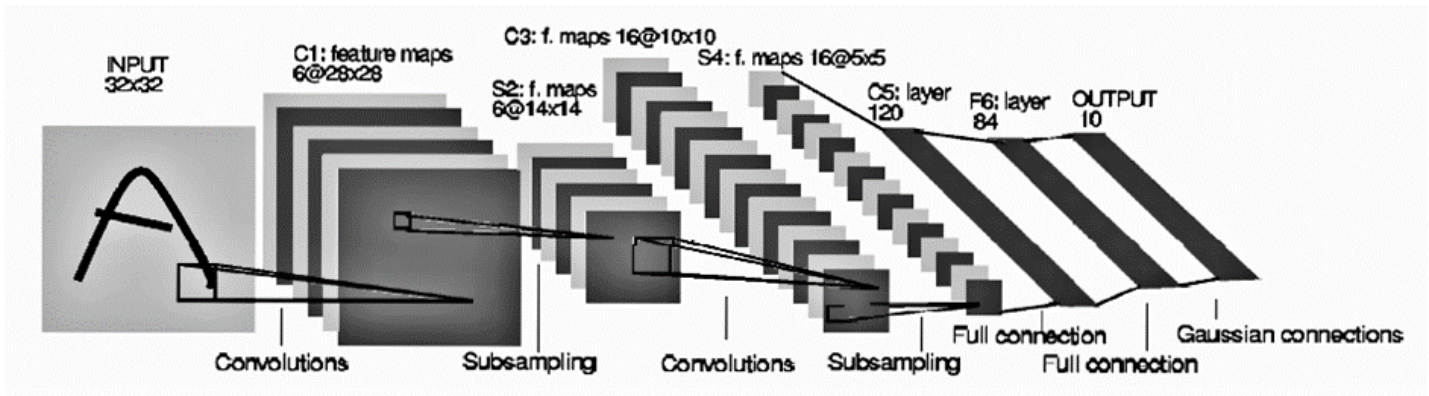
Fig. 1. Typical CNN(LeNet) [3]
