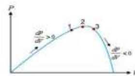
Fig. 3. P-V Characteristics of PV Panel
