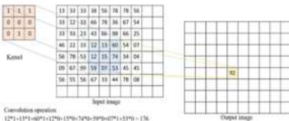
Fig 3: Image Classification
