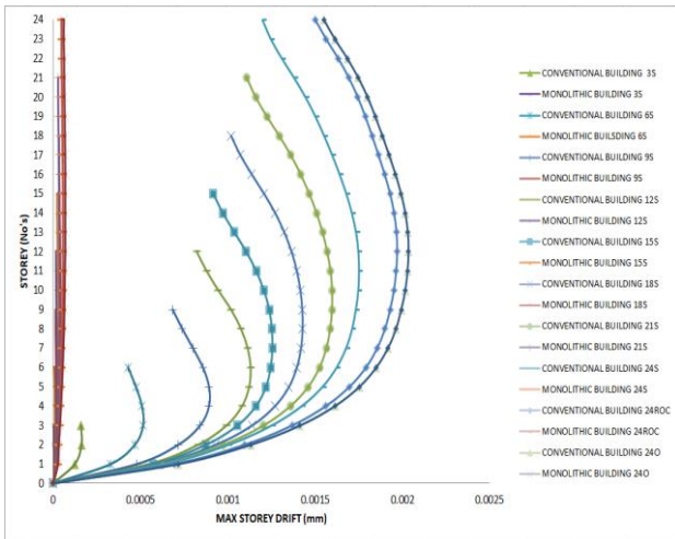
Chart 3: Variation in storey drift at every stage of construction - RS X
