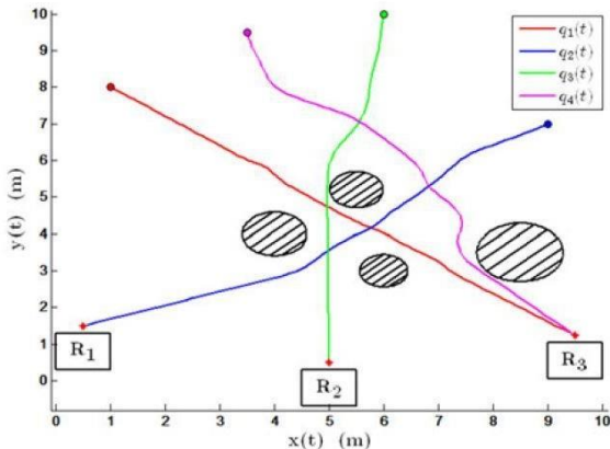
Figure 19: Path planning with obstacles (Demesure et al., 2017)
