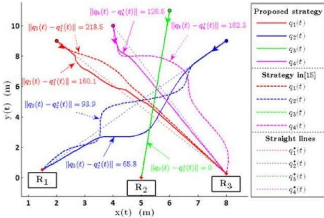
Figure 18: Graph of path planning simulation (Demesure et al., 2017)
