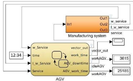
Figure 3: Matlab Simulink Model (Klosowski et al., 2018)
