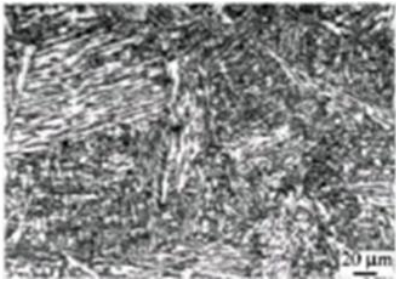
Fig.4.Welding microstructure map[11]
