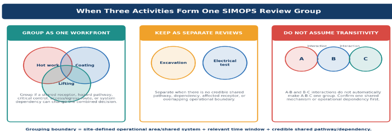
Figure 1A. Practical grouping boundary: when three activities form one shared SIMOPS review group and when pair reviews should remain separate.
