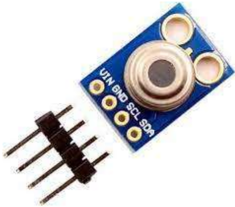
Figure 3: Image of a Temperature sensor MLX90614 src:- Circuit digest
