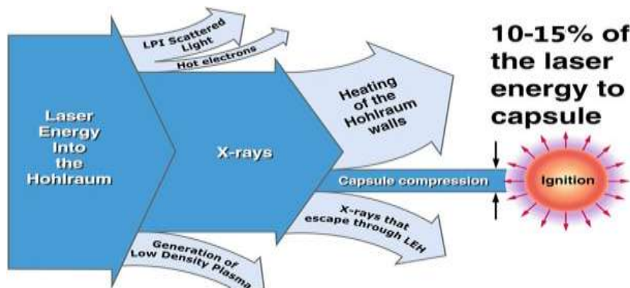
Figure (9): A schematic of where the laser energy goes for an indirect drive configuration. Only 10-15% of the laser energy makes it to the target in the form of X-rays.
