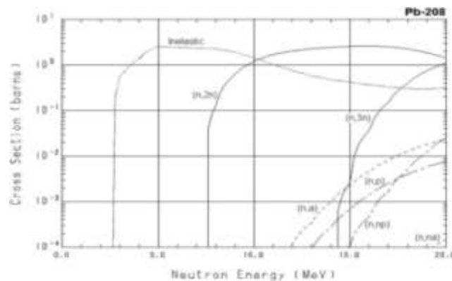
Figure (12). The cross sections for producing 1 or 2 additional neutrons in a lead target, as a function of the incident neutron energy.
