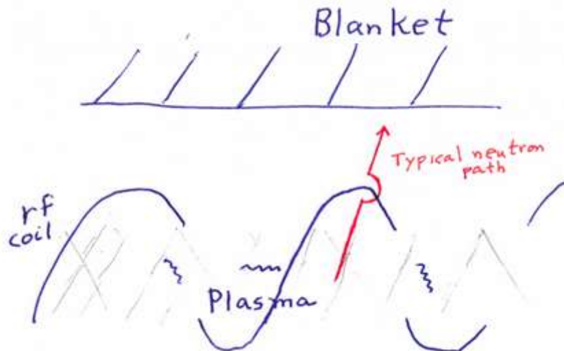
Figure (5): RF heater's view of fusion. Redrawn from memory from a collection of hand drawn cartoons and captions that Professor David Rose of MIT circulated in the 1960's and 1970's.
