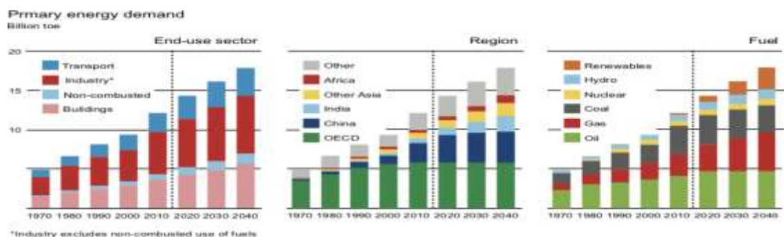
Figure (2): BP’s three graphs of energy demand by end use sector, region and fuel. The units are billions of tons of oil per year. Since this is an unusual unit for people not in the oil industry, we use terawatts (TW), where one terawatt is approximately one billion tons of oil per year.
