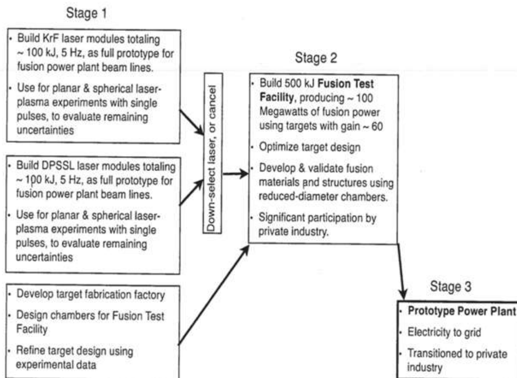
Figure (15): Steven Bodner's proposed plan for laser development for laser fusion.
