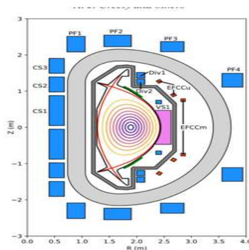
Figure (4): A schematic of the poloidal cross section of SPARC taken from Ref.(50). The pink part inside the vacuum chamber is the belt which carries the current rf current used for ion cyclotron heating.
