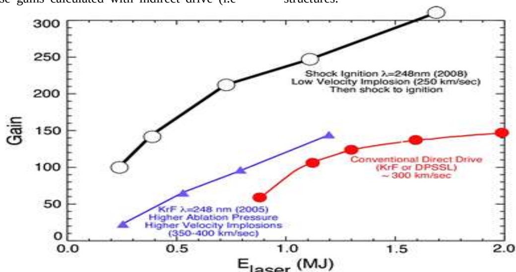
Figure (11): A variety of calculations of gain from NRL for direct drive laser fusion.
