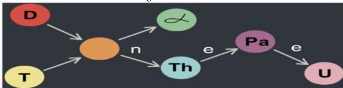
Figure 13: A schematic of the decay process where a fusion neutron is absorbed by a thorium nucleus, setting into motion a decay process which finally ends up as a ^{233}U nucleus; a perfectly good fuel for a thermal nuclear reactor.
