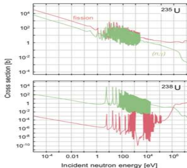
Figure 3 : The fission and neutron absorption cross section in barns (1 barn is 10^{-24} cm 2 ) for ^{235}\text{U} and ^{238}\text{U} as a function of the energy of the incident neutron. The cross sections look about the same for all fertile and fissile nuclei, depending whether their atomic number is odd or even.
