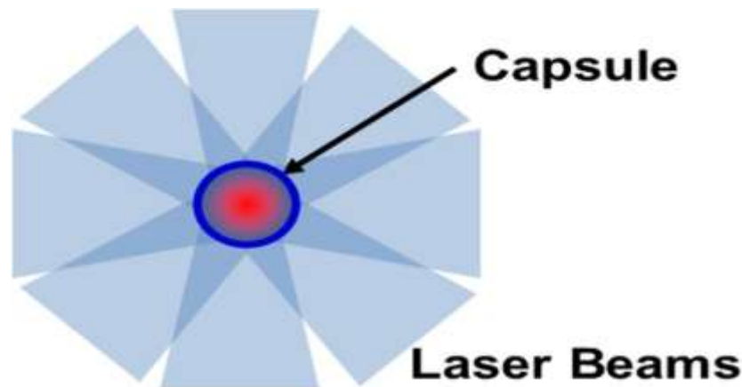
Figure (10): A schematic of direct drive laser fusion taken from Ref. (73). The laser beams directly hit the target, so very little energy is wasted in other loss channels, as is the case with indirect drive.
