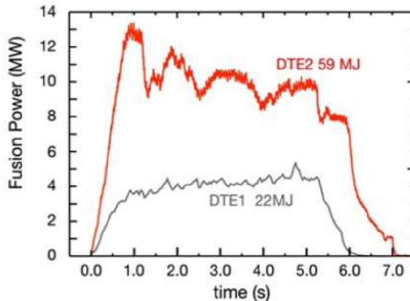
Figure (6): A plot of the fusion power in JET's most recent DT campaign compared to what it accomplished in 1997.
