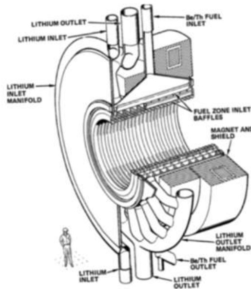
Figure 14: A schematic of a fusion breeding blanket surrounding a fusion reactor. Notice the input and exit pipes for the flowing lithium and thorium.
