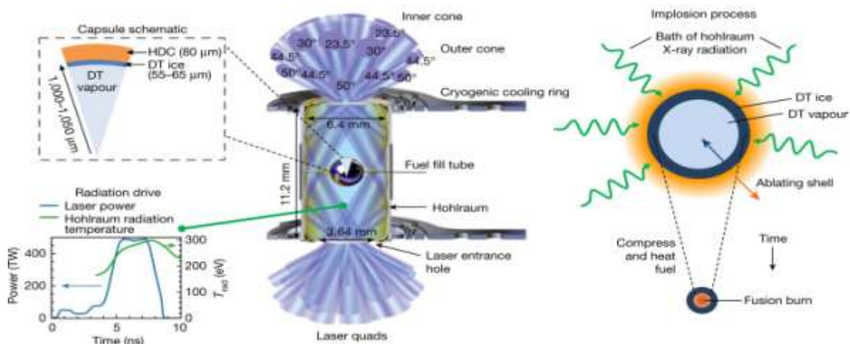
Figure (8): A schematic of the LLNL approach to laser fusion taken from Ref(71).
