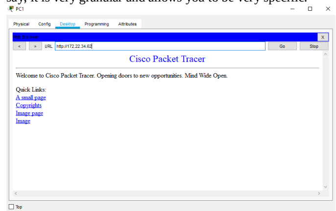
Fig. 8 Allowing access for http application
