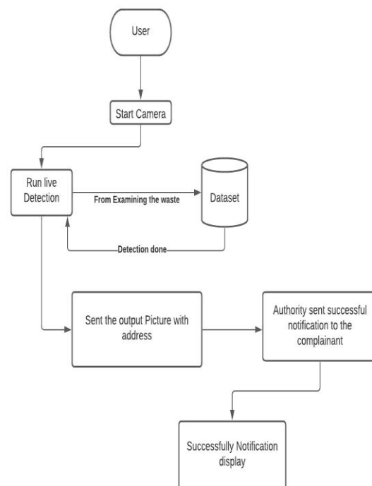
Fig.3. Architecture Diagram
