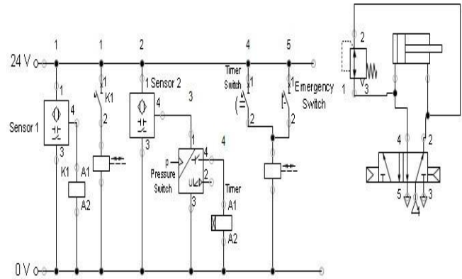
Fig. 2. AGC electro-pneumatic circuit on FluidSim
