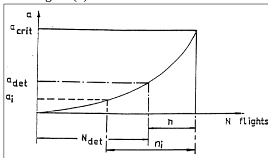
Fig (1) Definition of Fatigue crack propagation life term. [6]
