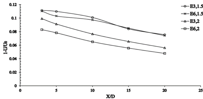
Figure 4: Longitudinal variation of velocity deficit downstream of the array
