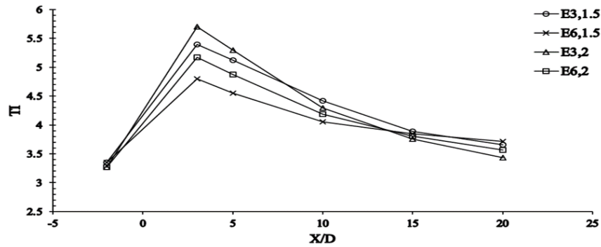
Figure 5: Longitudinal variation of turbulence intensity
