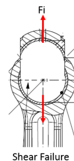
Figure 7. Shearing of connecting rod Small end
