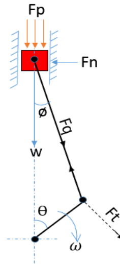
Figure 2. Slider Crank Mechanism for Connecting rod. ....[2]
