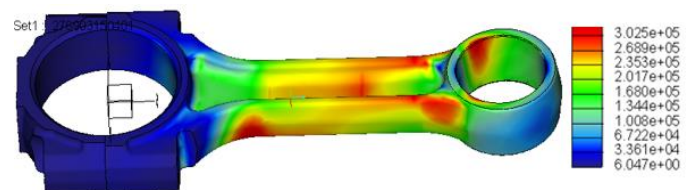
Figure 9. Stresse in KPa.
