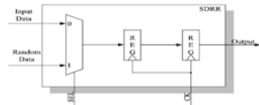
Fig.2.2.SDRR Architecture
