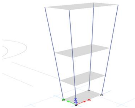
Fig 1. Steel frame
