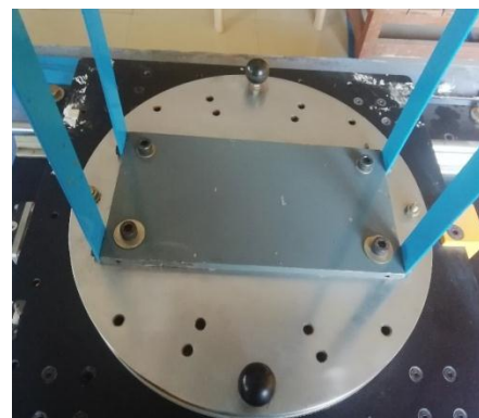
Fig 9: Bottom plate connected to shake table
