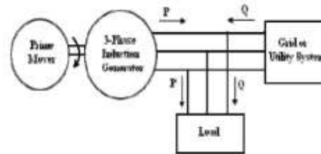
Figure: 1. Grid Connected Induction Generator
