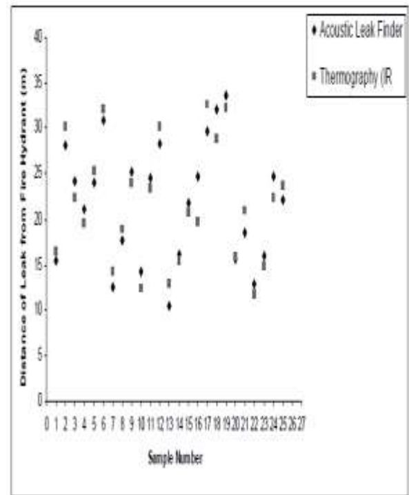
Figure 4: Leak Locations (m) using Acoustic Leak Finder Verses IR camera
