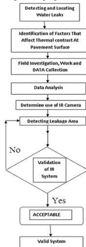
Figure 1: Proposed Methodology
