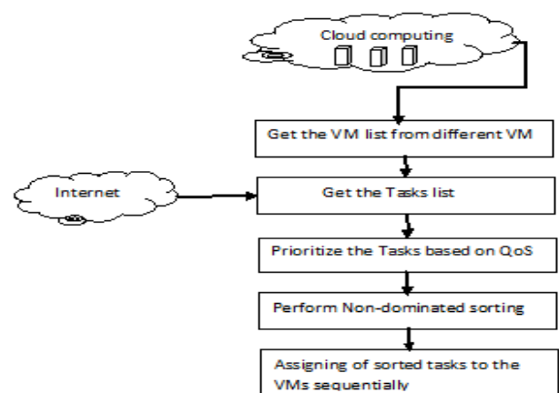
Fig. 1. Multi-Objective task scheduling and dominance relation
