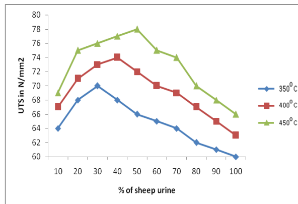
Fig.1. ( % of Sheep urine Vs UTS of Al 2585)
