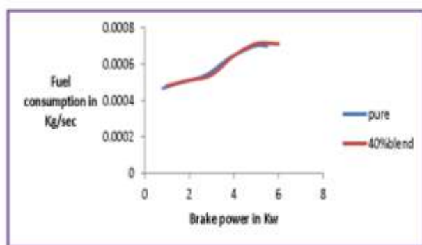
Fig. 7. Fuel Consumption Vs Brake Power
