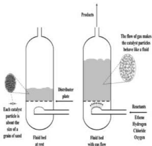
Fig. 1. Diagram of fluidized bed reactor [22].
