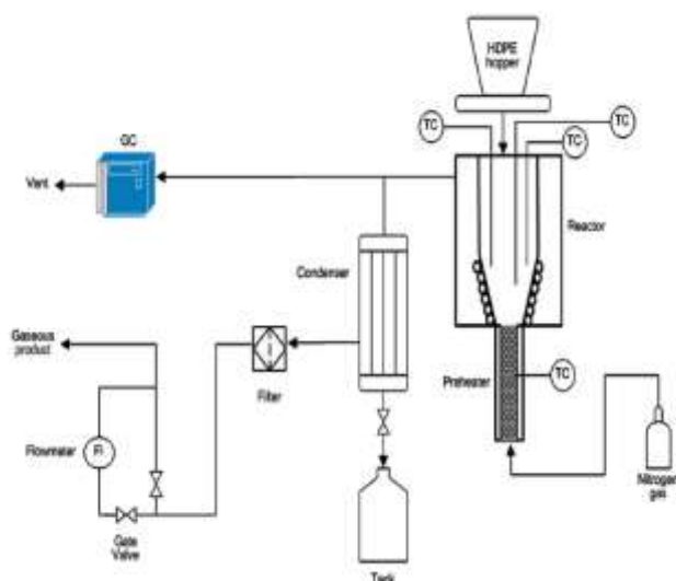
Fig. 2. Diagram of CSBR in HDPE pyrolysis using zeolite catalyst [23].
