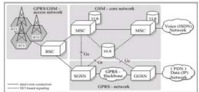
Figure:2 2.5G Architecture Model
