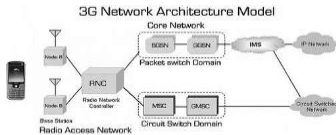
Figure:3 3G architecture model
