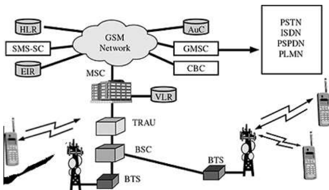
Figure:1 2G Architecture Model.
