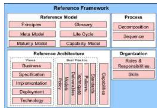
Fig. 2: The Framework of Cloud Computing
