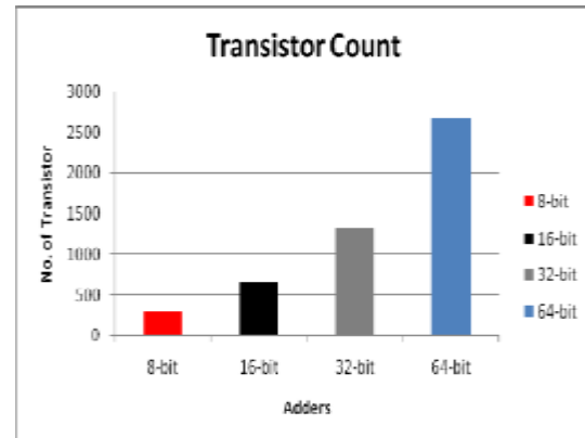
Figure 9. Number of Transistors
