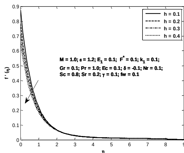
Fig. 30: Velocity profiles for different Values of h
