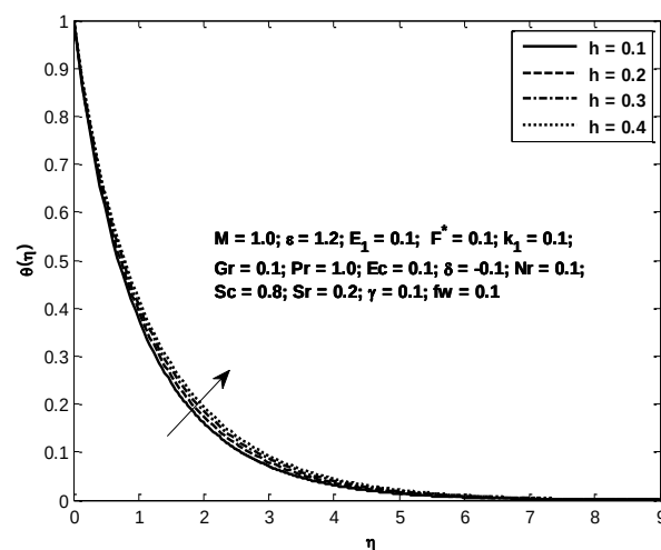
Fig. 31: Temperature profiles for different values of h
