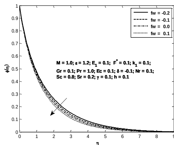
Fig. 29: Concentration profiles for different values of fw
