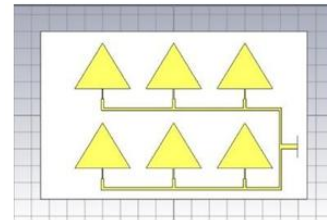
Figure 3.4: 6-element quarter wave feed array antenna
