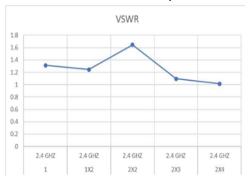
Figure 4.3.3: VSWR of quarter wave feed array antennas
