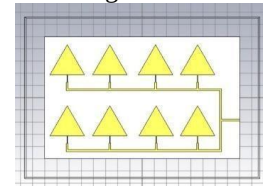
Figure 3.4: 8-element quarter wave feed array antenna
