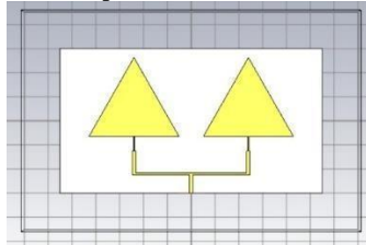
Figure 3.2: 2-element quarter wave feed array antenna
