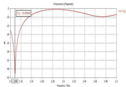
Figure 4.1.2: S-parameter or return loss of 8 element quarter wave array.
