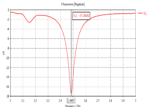
Figure 4.1.1: S-parameter of 1 element quarter wave feed
