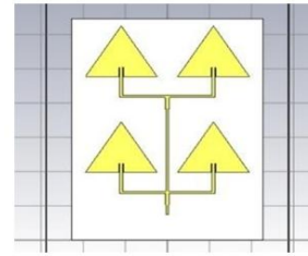
Figure 3.3: 4-element quarter wave feed array antenna
