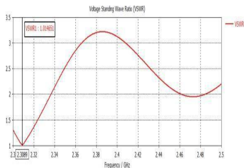
Figure 4.3.2: VSWR for 8 element quarter wave arrays.
