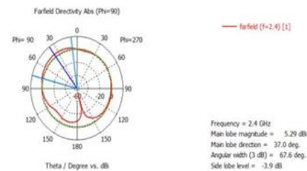
Figure 4.3.3: Antenna pattern of single quarter wave feed
