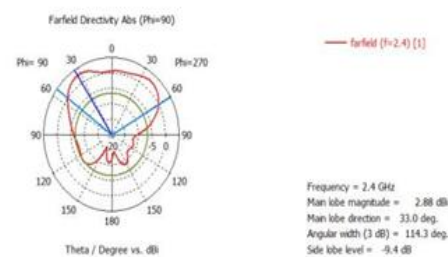
Figure 4.3.3: Antenna pattern of 8 quarter wave feed\
