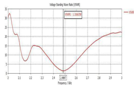
Figure 4.3.1: VSWR for 1 element quarter wave array.
