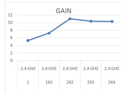
Figure 4.2.3: GAIN of quarter wave feed array antennas
