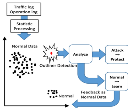
Figure 1: Flow of cyber attack detection system
