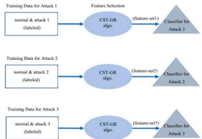
Figure 3: The training phase (the case of three classifiers). CST-GR, correlated set thresholding on gain-ratio.
