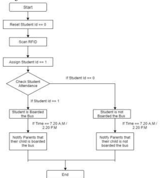
Figure.13 Attendance Checker Flowchart
