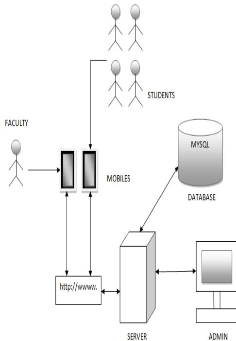
Fig.1. Architectural Design
