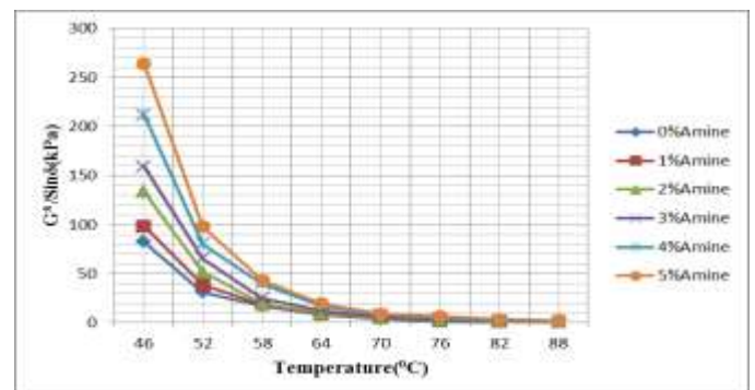
Fig. 10. Effect of amine on rutting resistance parameter
