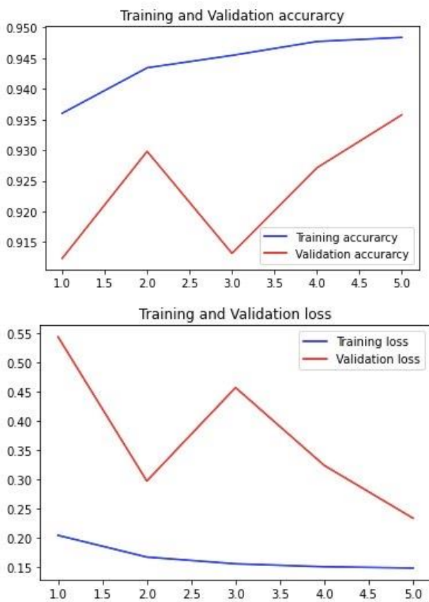
Fig.10. Training and Validation loss and accuracy
