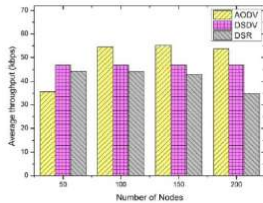
Fig 2. Throughput of AODV, DSDV and DSR
