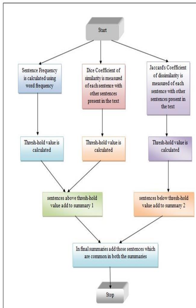
Fig. 1. Basic workflow of Algorithm
