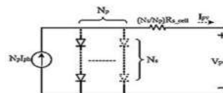
Fig. 1. Multi-diode model
