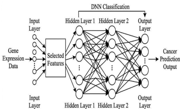
Fig. 3. Architecture of Deep Neural Network classifier [11].
