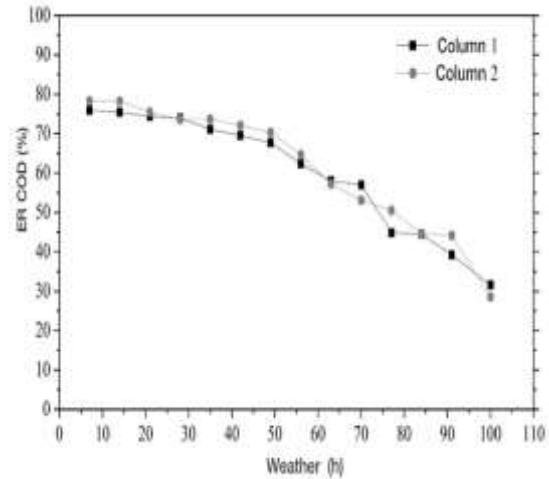
Figure 8. DQO removal efficiency curve in columns packed with CA6
